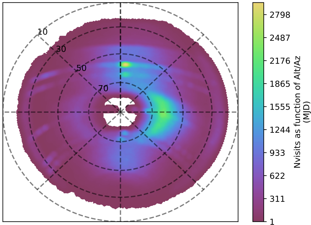
no_long_daily_v3.4_10yrs i band: Nvisits as function of Alt/Az
