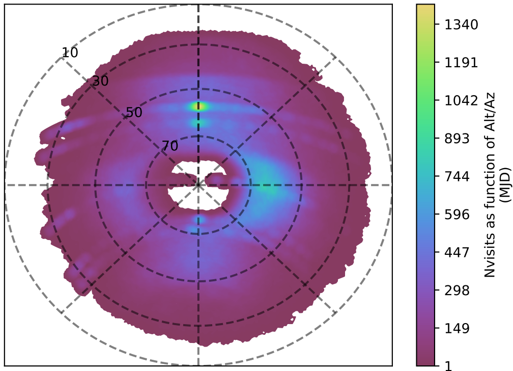
no_long_daily_v3.4_10yrs g band: Nvisits as function of Alt/Az
