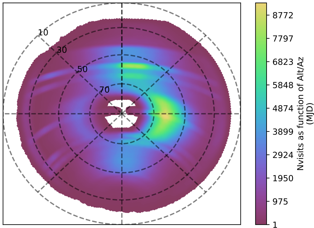
no_long_daily_v3.4_10yrs all bands: Nvisits as function of Alt/Az
