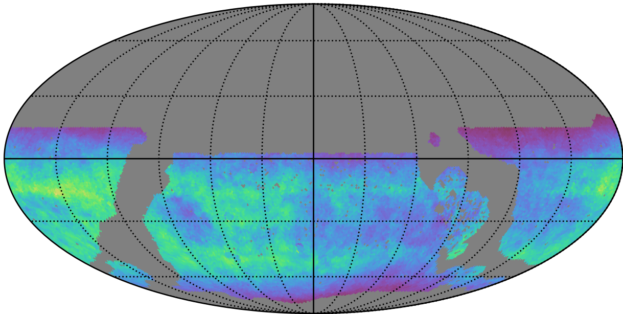
no_long_daily_v3.4_10yrs WFD u band: Normalized Teff
