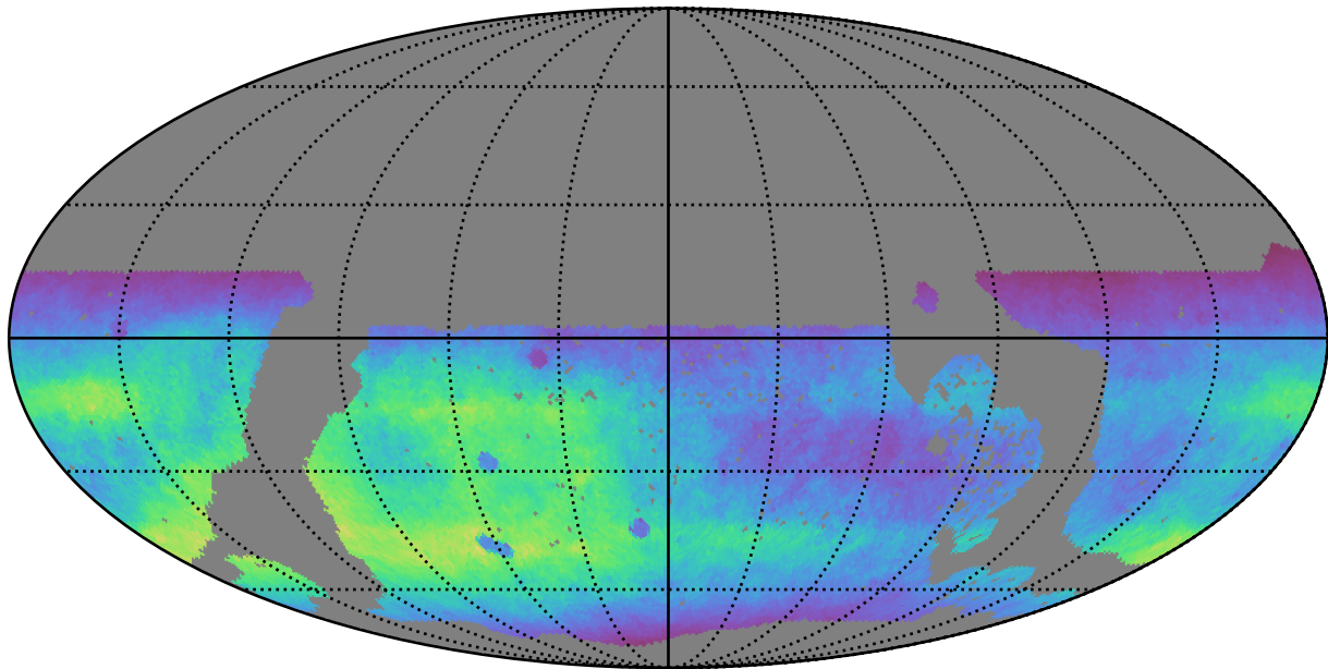
no_long_daily_v3.4_10yrs WFD r band: Normalized Teff
