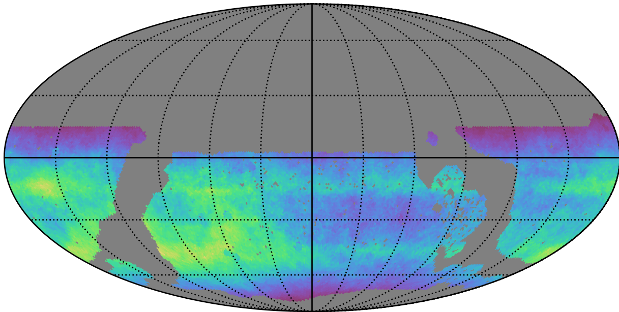
no_long_daily_v3.4_10yrs WFD i band: Normalized Teff
