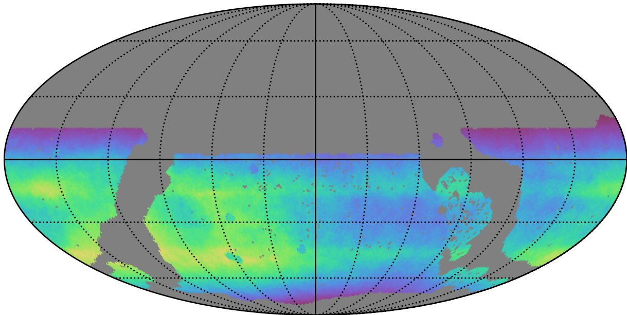
no_long_daily_v3.4_10yrs WFD all bands: Normalized Teff
