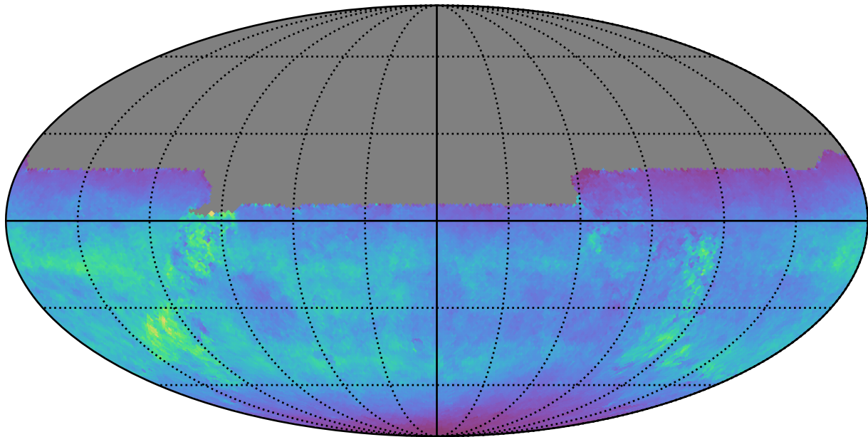
no_long_daily_v3.4_10yrs All sky u band: Normalized Teff
