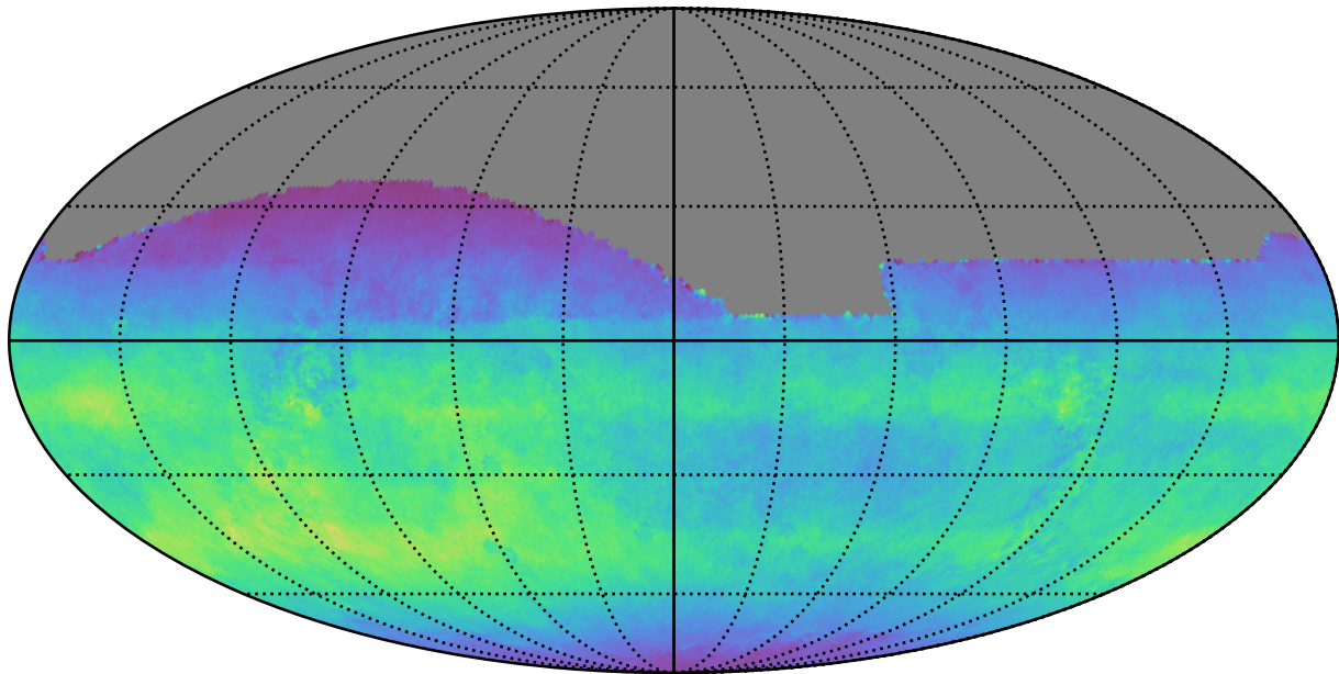
no_long_daily_v3.4_10yrs All sky i band: Normalized Teff
