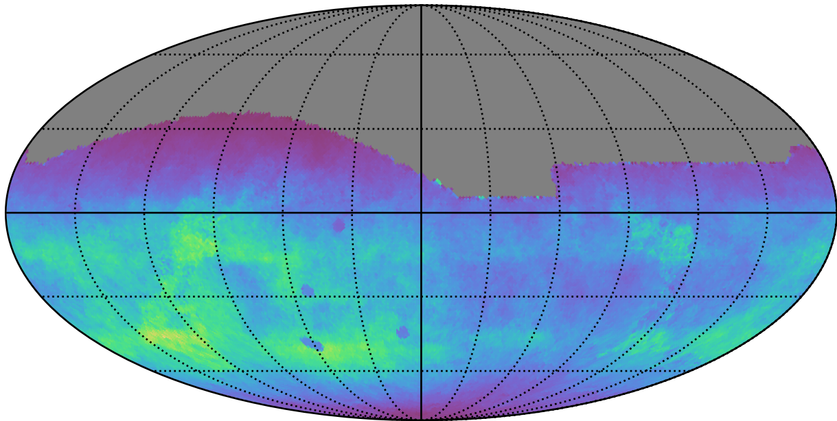
no_long_daily_v3.4_10yrs All sky g band: Normalized Teff
