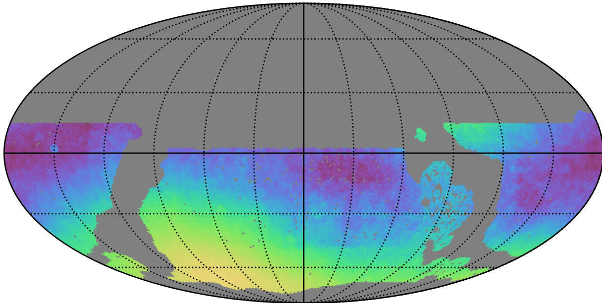
no_long_daily_v3.4_10yrs WFD: Normalized Parallax Uncert @ 24.0
