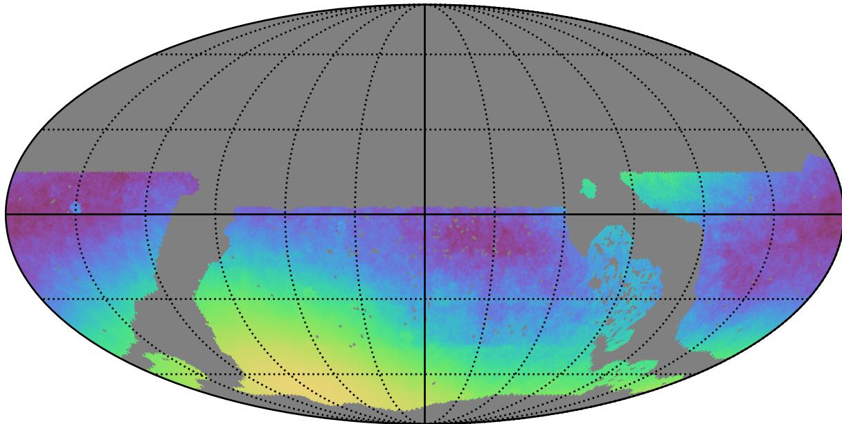
no_long_daily_v3.4_10yrs WFD: Normalized Parallax Uncert @ 22.4
