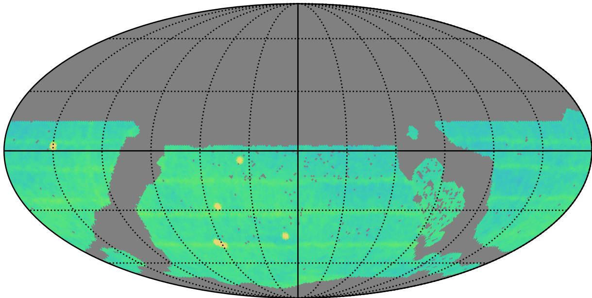
no_long_daily_v3.4_10yrs WFD all bands: N Unique Nights
