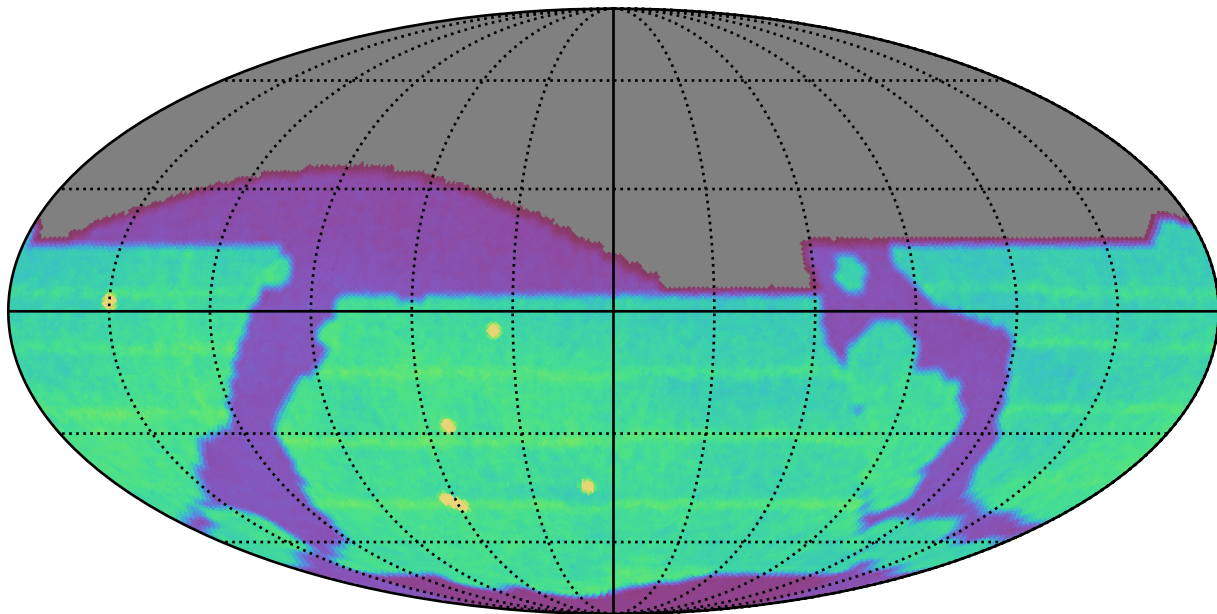
no_long_daily_v3.4_10yrs All sky all bands: N Unique Nights
