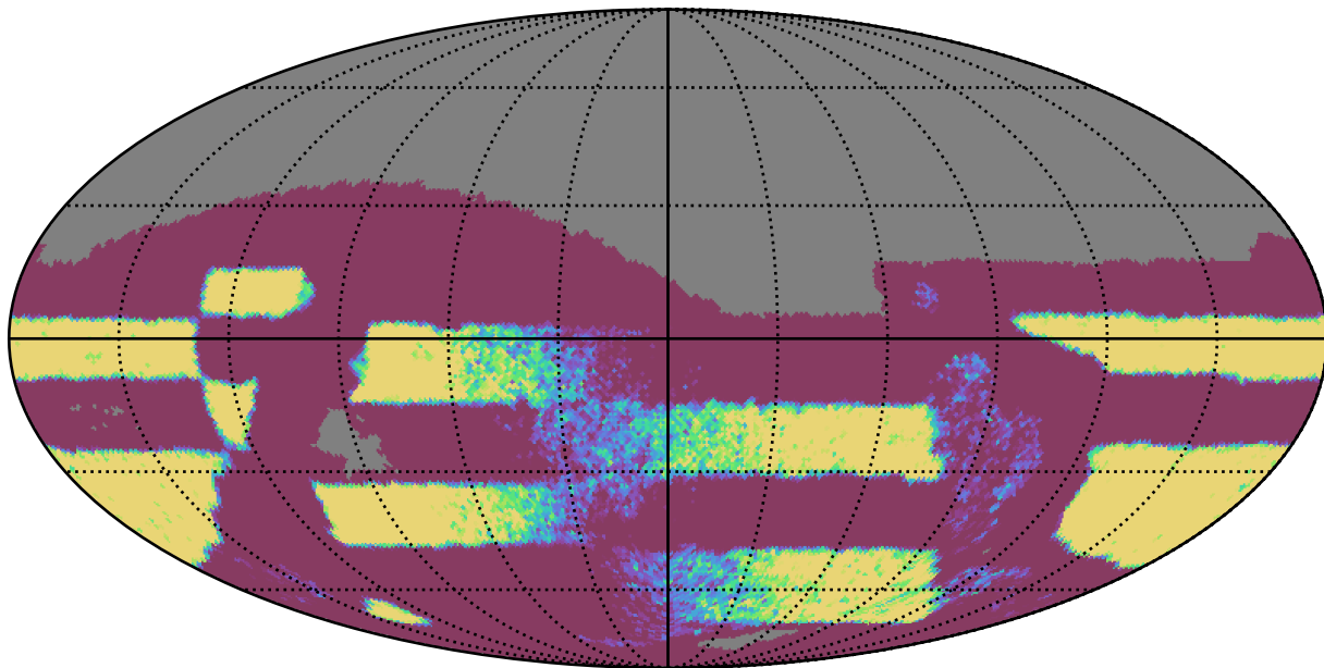
no_long_daily_v3.4_10yrs Yr 3-4 all bands: NVisits
