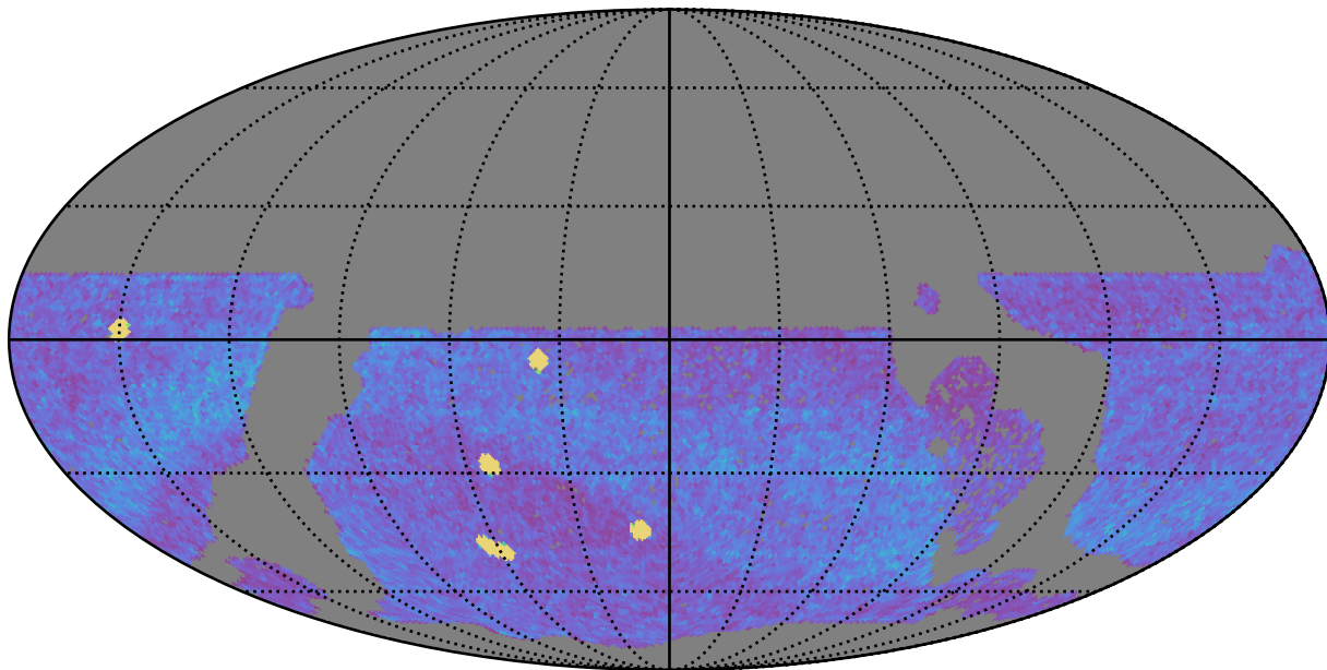
no_long_daily_v3.4_10yrs WFD all bands: NVisits
