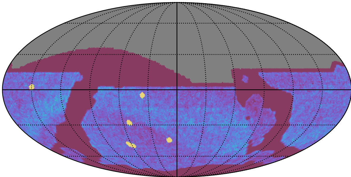
no_long_daily_v3.4_10yrs All sky all bands: NVisits
