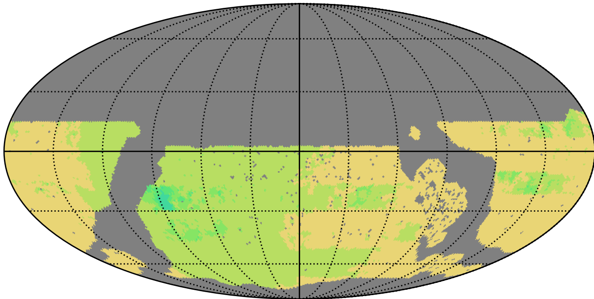
no_long_daily_v3.4_10yrs WFD all bands: NSeasons
