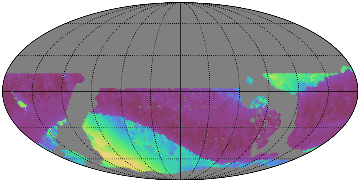
no_long_daily_v3.4_10yrs WFD all bands: Min solarElong
