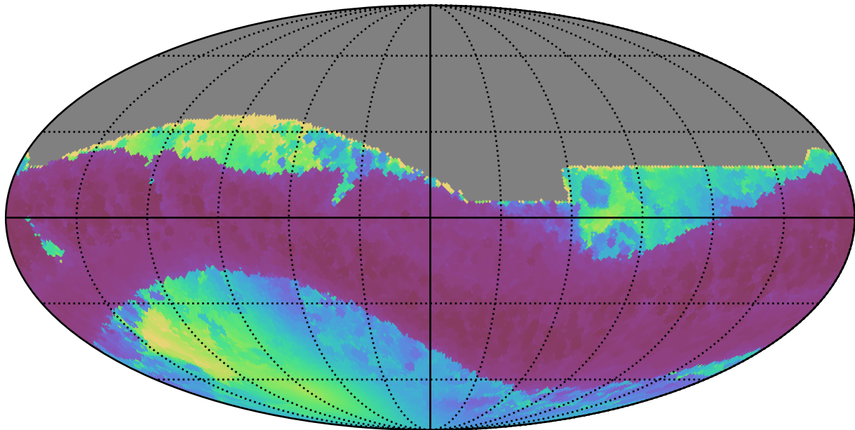
no_long_daily_v3.4_10yrs All sky all bands: Min solarElong
