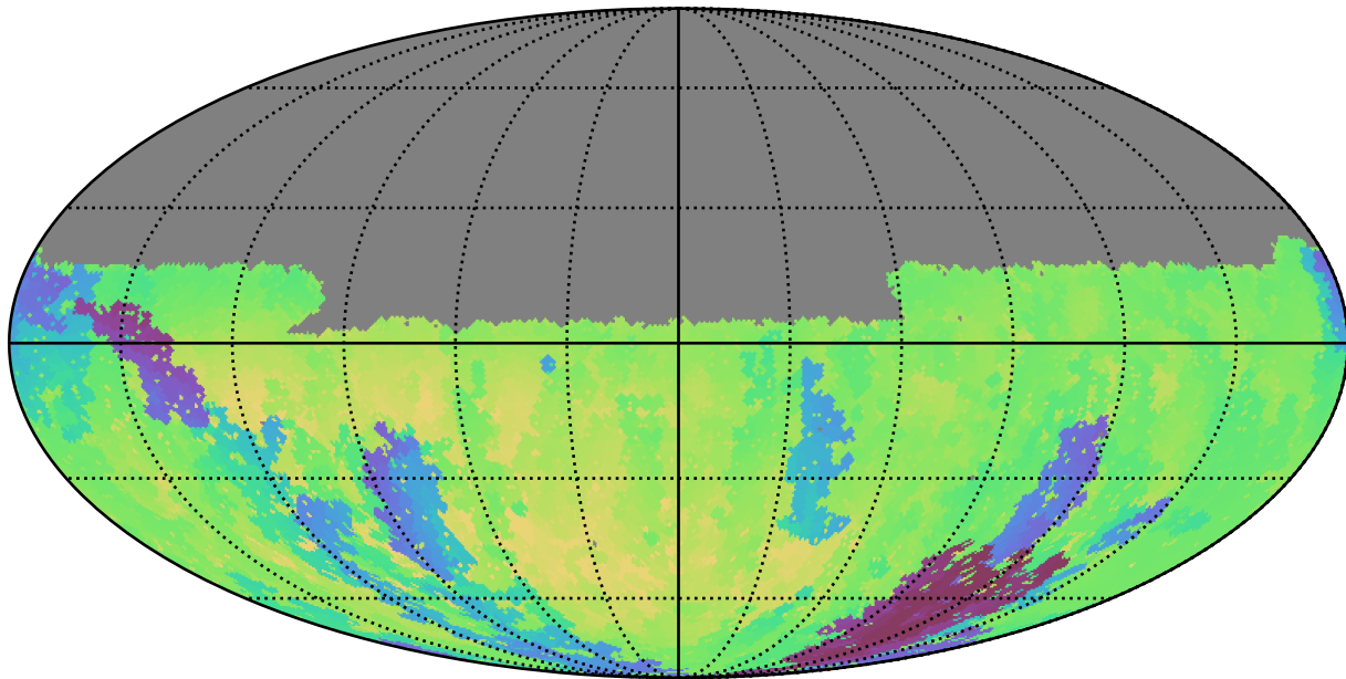
no_long_daily_v3.4_10yrs Yr 1 u band: Min skyBrightness
