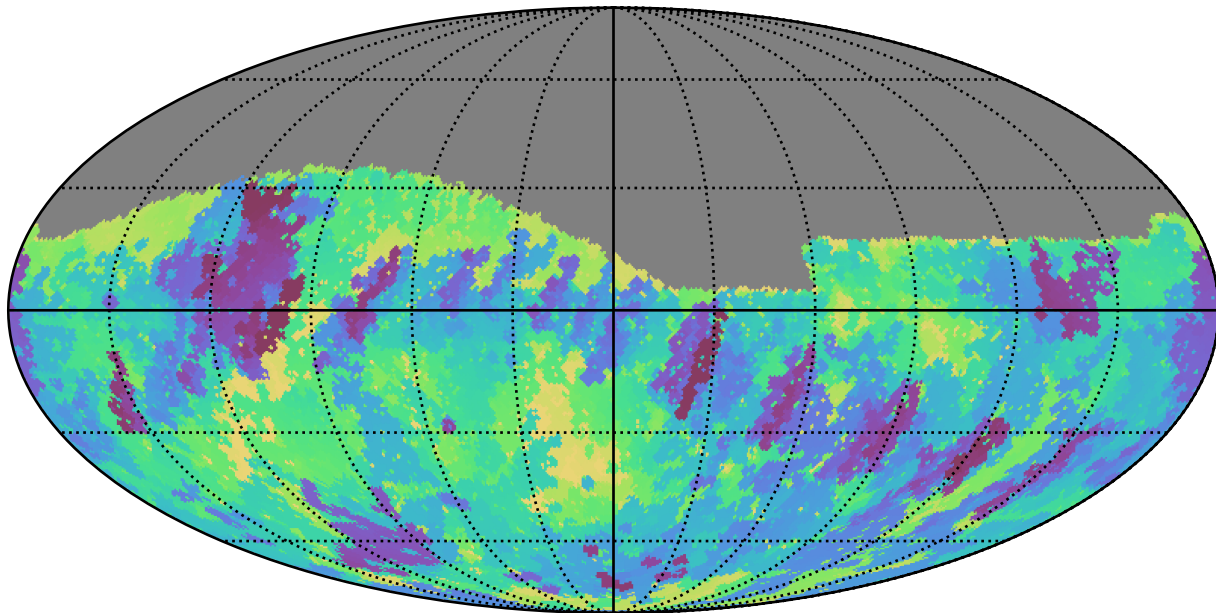
no_long_daily_v3.4_10yrs Yr 1 r band: Min skyBrightness
