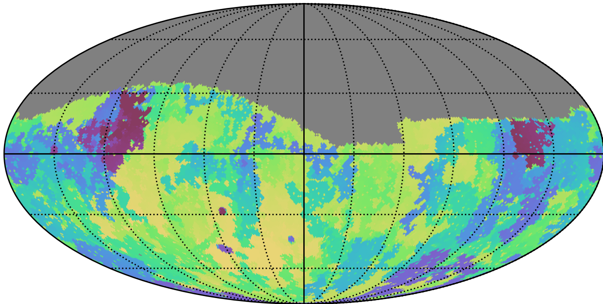
no_long_daily_v3.4_10yrs Yr 1 g band: Min skyBrightness
