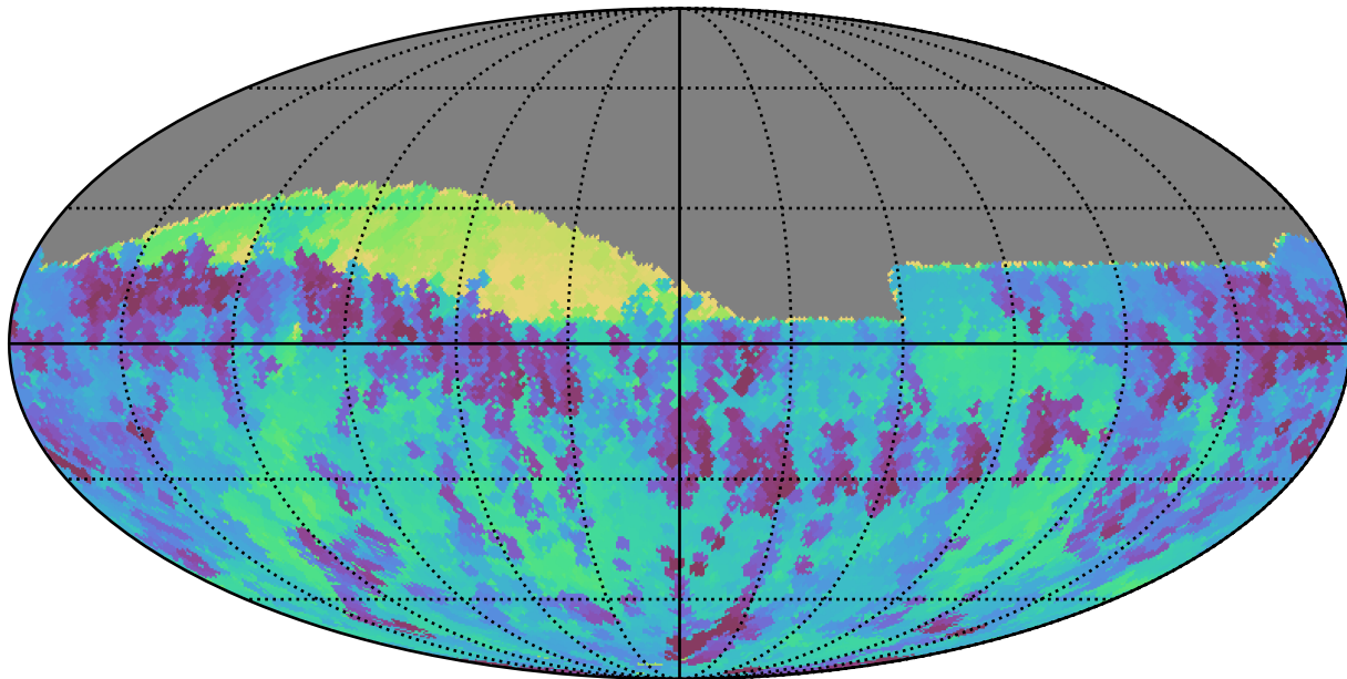
no_long_daily_v3.4_10yrs Yr 1 all bands: Min skyBrightness
