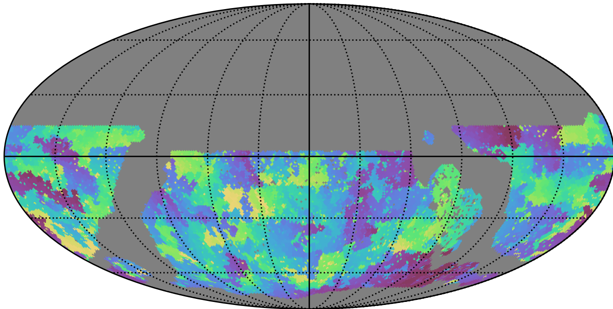
no_long_daily_v3.4_10yrs WFD u band: Min skyBrightness
