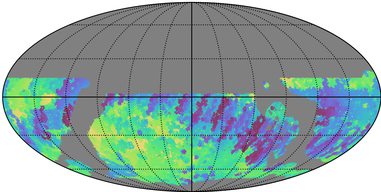
no_long_daily_v3.4_10yrs WFD r band: Min skyBrightness
