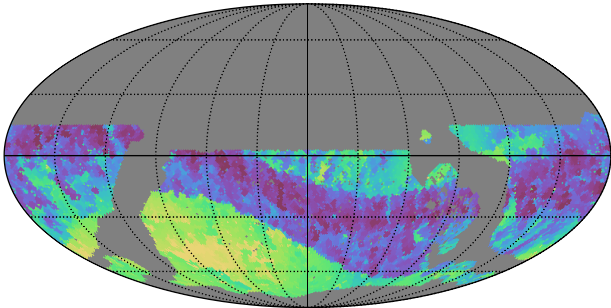
no_long_daily_v3.4_10yrs WFD i band: Min skyBrightness
