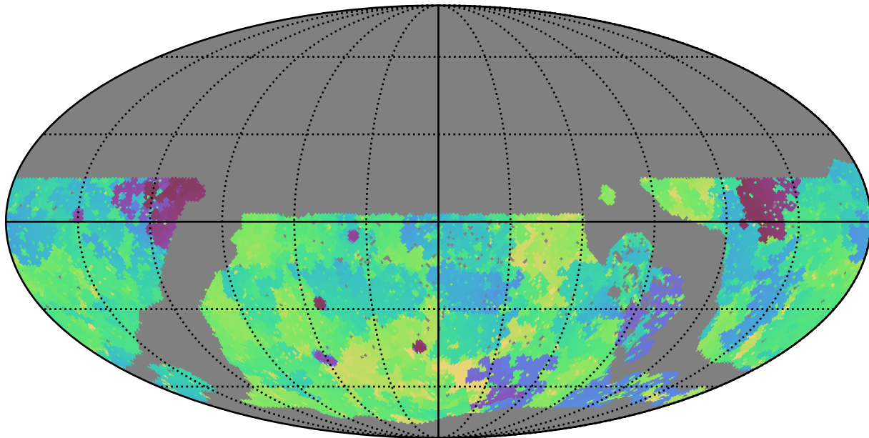
no_long_daily_v3.4_10yrs WFD g band: Min skyBrightness
