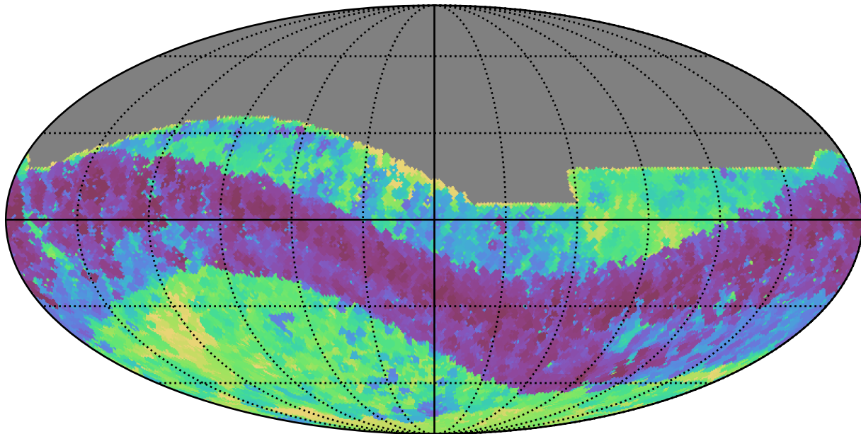
no_long_daily_v3.4_10yrs All sky z band: Min skyBrightness
