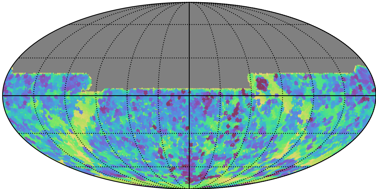
no_long_daily_v3.4_10yrs All sky y band: Min skyBrightness
