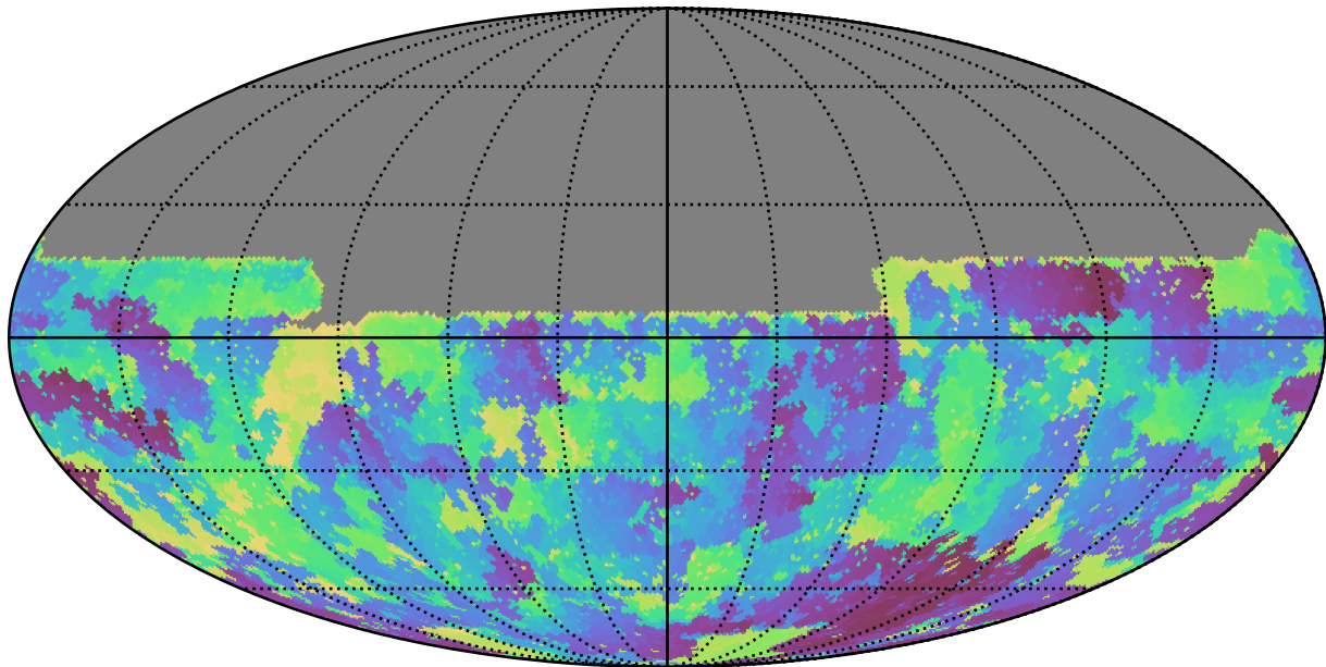
no_long_daily_v3.4_10yrs All sky u band: Min skyBrightness
