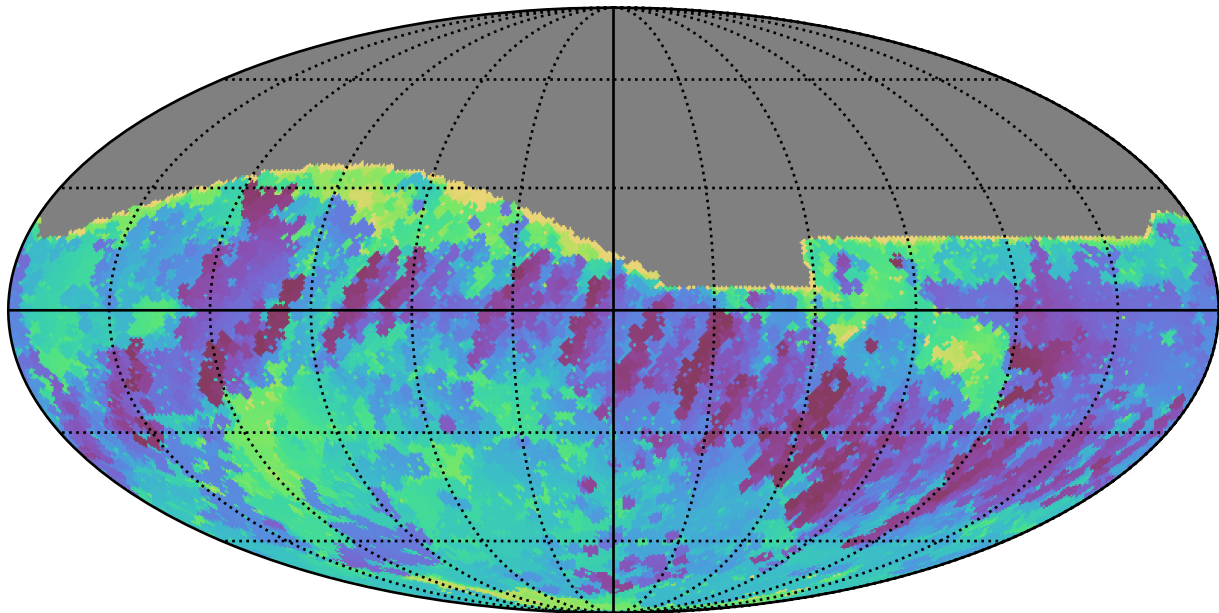
no_long_daily_v3.4_10yrs All sky r band: Min skyBrightness
