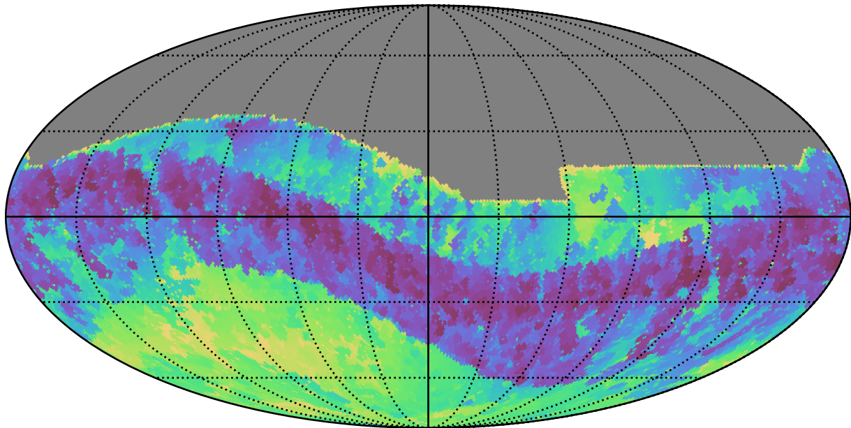
no_long_daily_v3.4_10yrs All sky i band: Min skyBrightness
