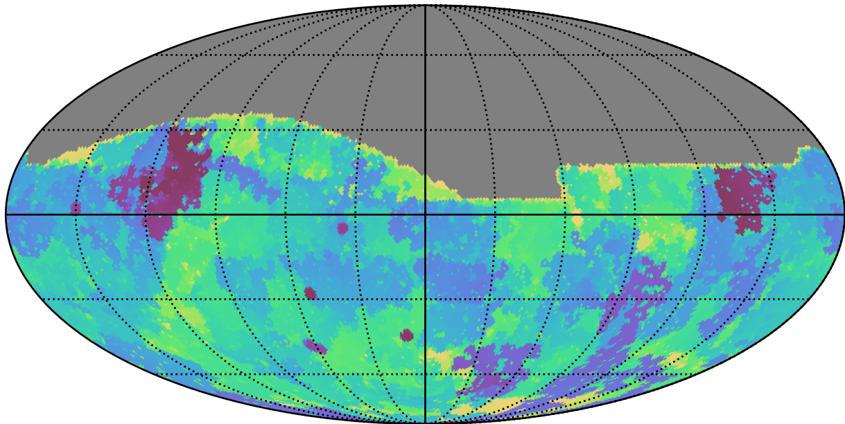
no_long_daily_v3.4_10yrs All sky g band: Min skyBrightness
