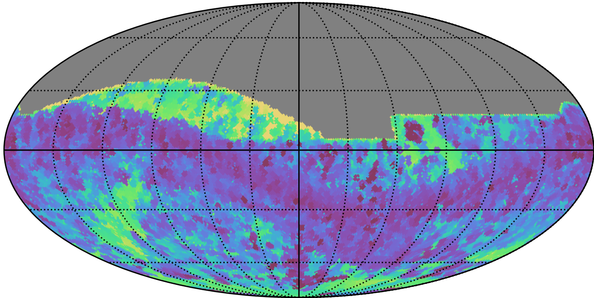
no_long_daily_v3.4_10yrs All sky all bands: Min skyBrightness
