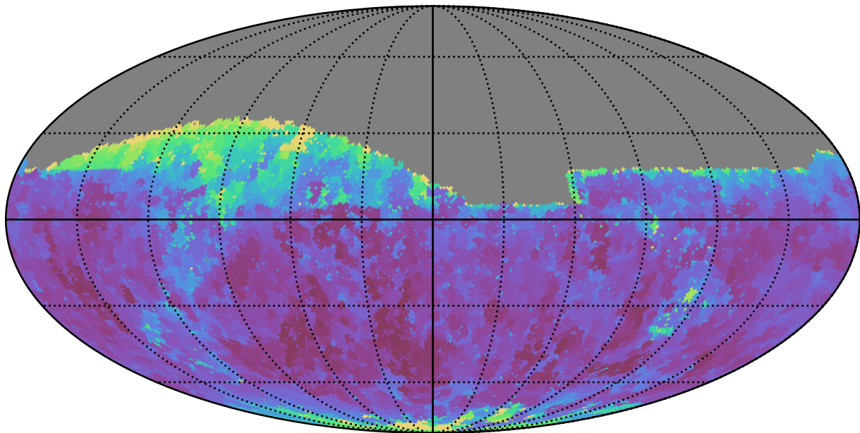
no_long_daily_v3.4_10yrs Yr 1 z band: Min seeingEff
