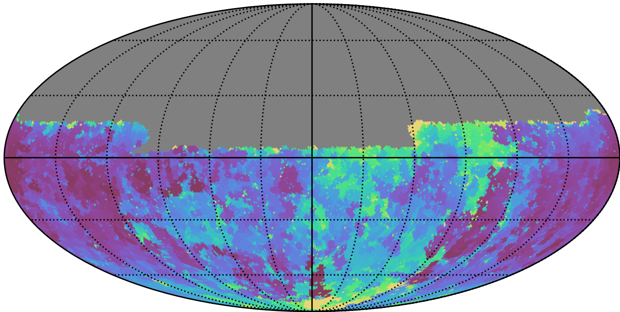
no_long_daily_v3.4_10yrs Yr 1 u band: Min seeingEff
