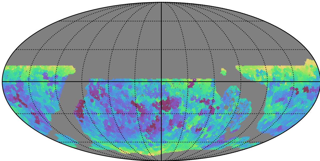
no_long_daily_v3.4_10yrs WFD z band: Min seeingEff
