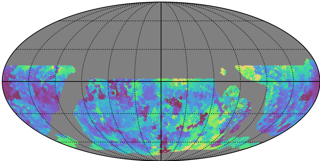
no_long_daily_v3.4_10yrs WFD u band: Min seeingEff
