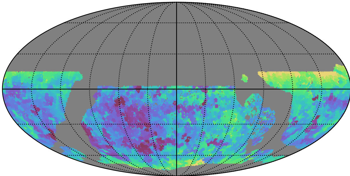
no_long_daily_v3.4_10yrs WFD r band: Min seeingEff
