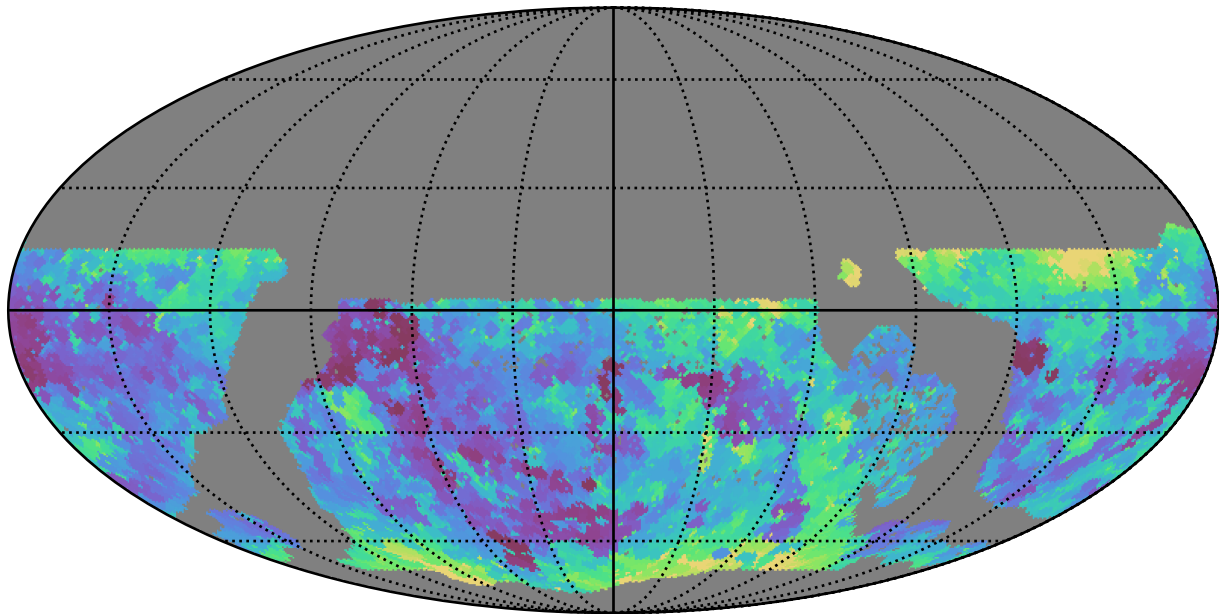
no_long_daily_v3.4_10yrs WFD g band: Min seeingEff
