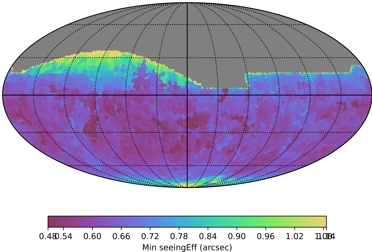
no_long_daily_v3.4_10yrs All sky z band: Min seeingEff
