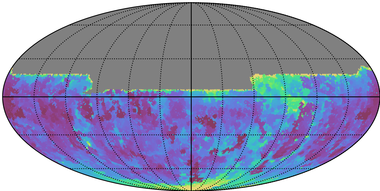
no_long_daily_v3.4_10yrs All sky u band: Min seeingEff
