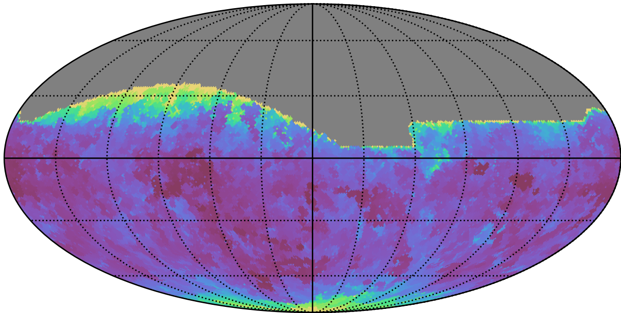
no_long_daily_v3.4_10yrs All sky g band: Min seeingEff
