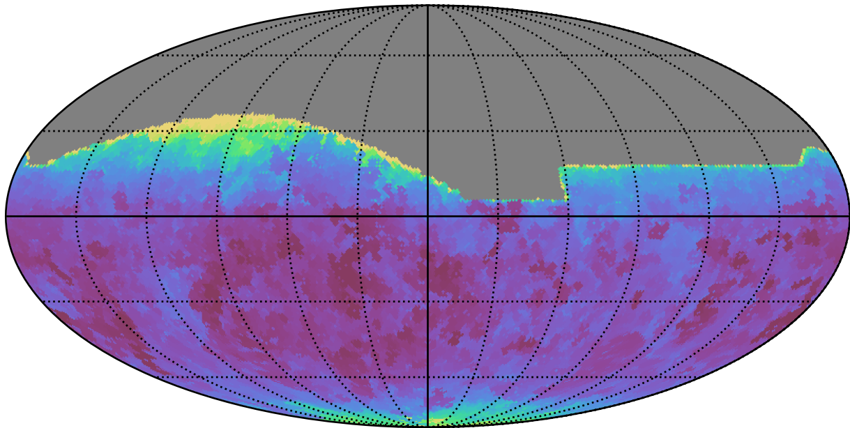
no_long_daily_v3.4_10yrs All sky all bands: Min seeingEff
