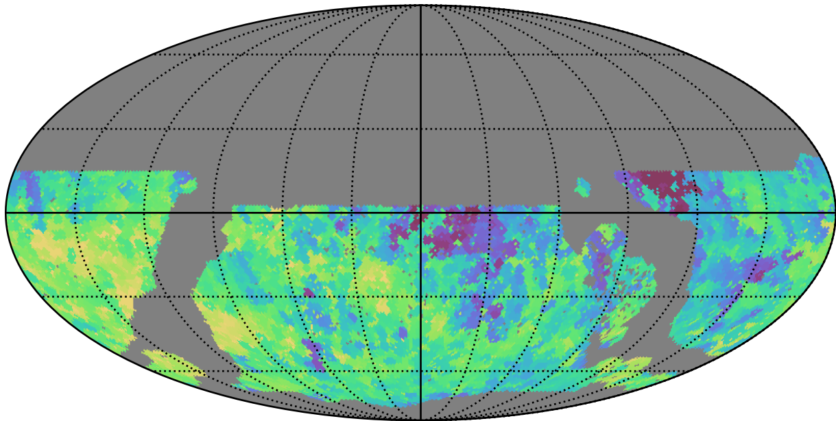
no_long_daily_v3.4_10yrs WFD all bands: Min saturation_mag
