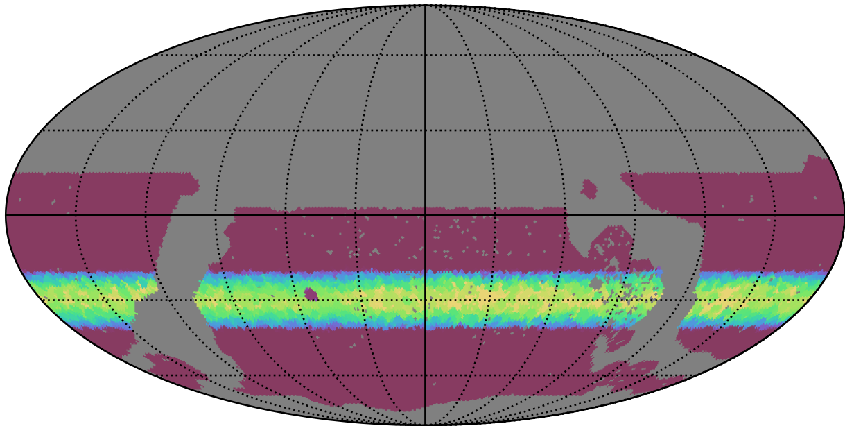
no_long_daily_v3.4_10yrs WFD all bands: Min normairmass
