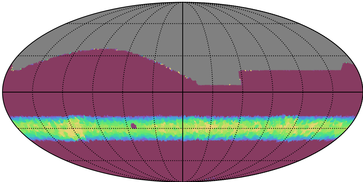
no_long_daily_v3.4_10yrs All sky all bands: Min normairmass
