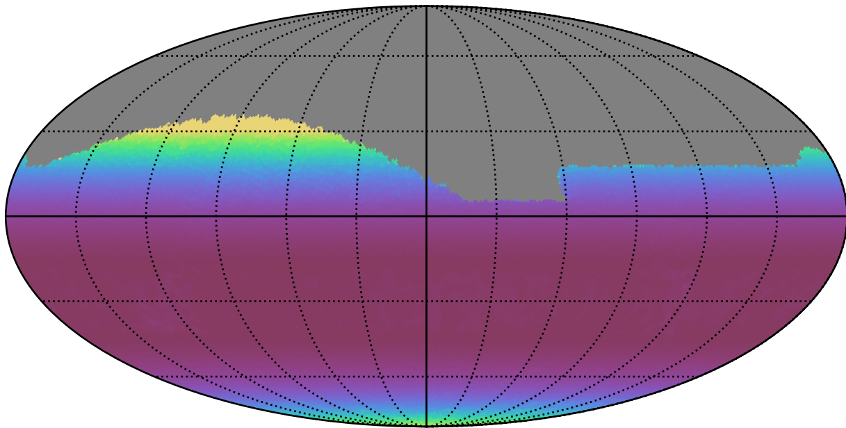
no_long_daily_v3.4_10yrs Yr 1 all bands: Min airmass
