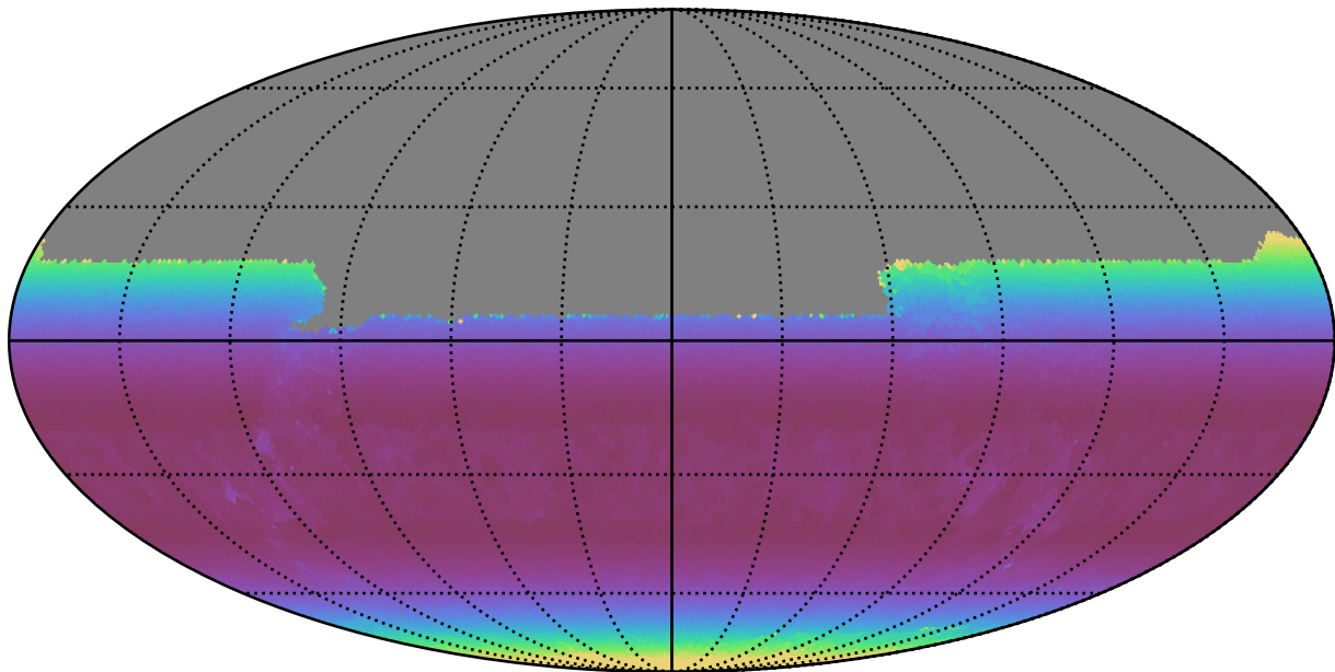
no_long_daily_v3.4_10yrs All sky u band: Min airmass
